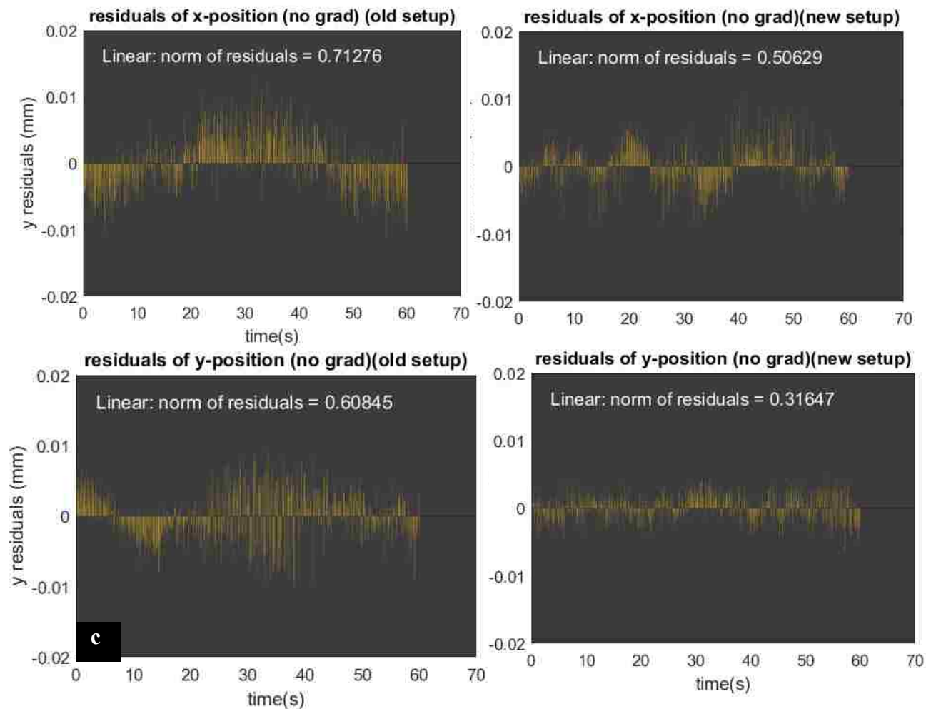
Figure 5.2 X and Y positions of recorded moving pattern without scan. a) X position of old design b) X position of new design c) Y position of old design d) Y position of new design
